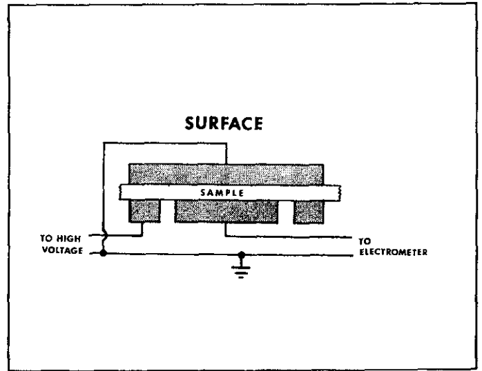
FIGURE 5. SURFACE RESISTIVITY
