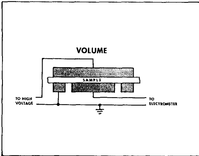
FIGURE 4. VOLUME RESISTIVITY
